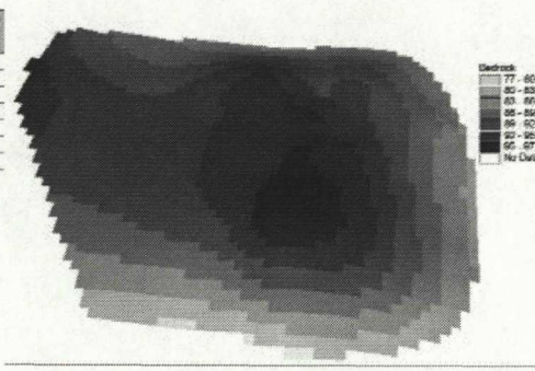
Figure 4 Bedrock DTM (res. 5m)
