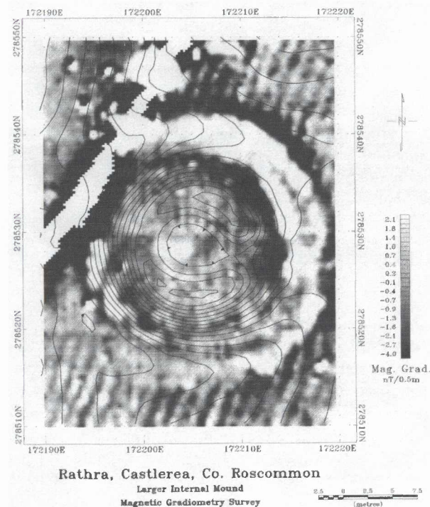
Fig. 8. A grey-scale magnetic gradiometry image of the larger internal mound at Rathra with an overlay of topographical contours at 0.25m intervals (Geosoft software)
