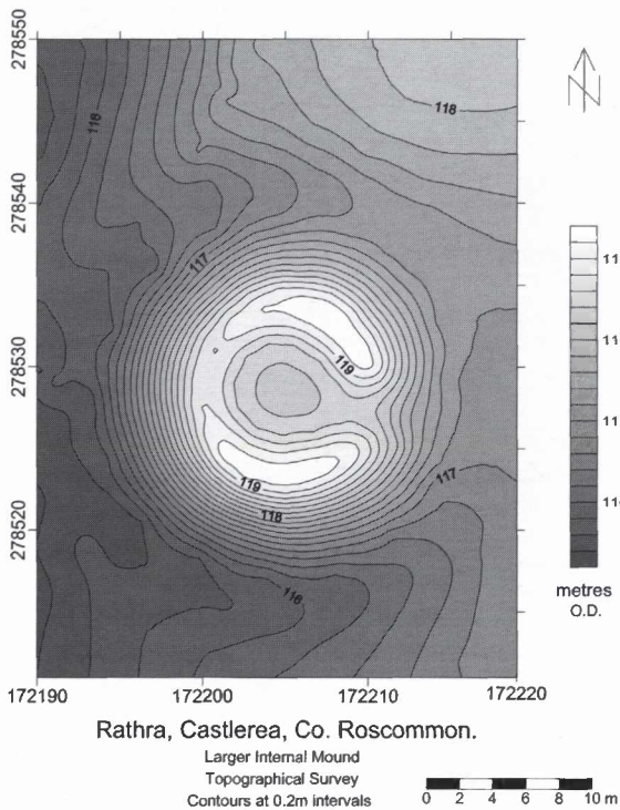
Fig. 6. A topographical contour map (0.2m contours) of the larger internal mound at Rathra (Surfer software)
