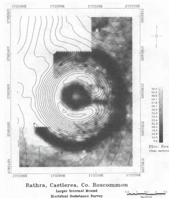
Fig. 9. A grey-scale electrical resistance image of the larger internal mound at Rathra with an overlay of topographical contours at 0.25m intervals (Geosoft Software)
