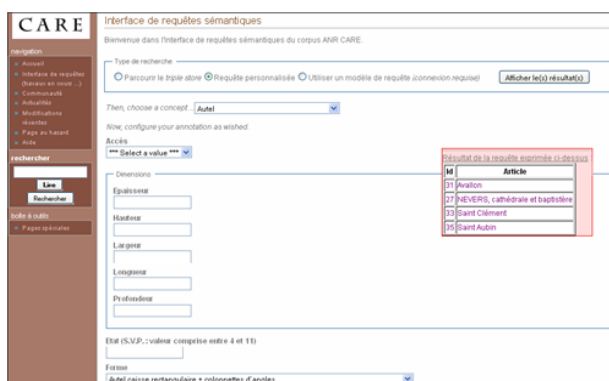
Figure 7: Query Interface.
