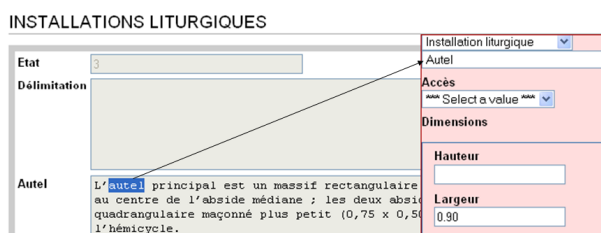
Figure 6: Annotation interface.
