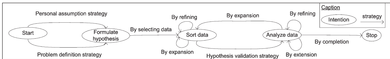
Figure 7. Strategy-oriented process model describing the analysis of data.
