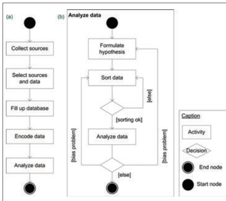
Figure 3. Activity-oriented process model describing the analysis of data.
