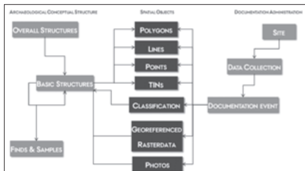
Figure 1. The data structure. The division into three columns allow three different entry points of data exploration.
