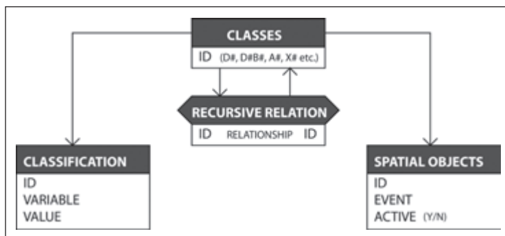
Figure 3. The database model.
