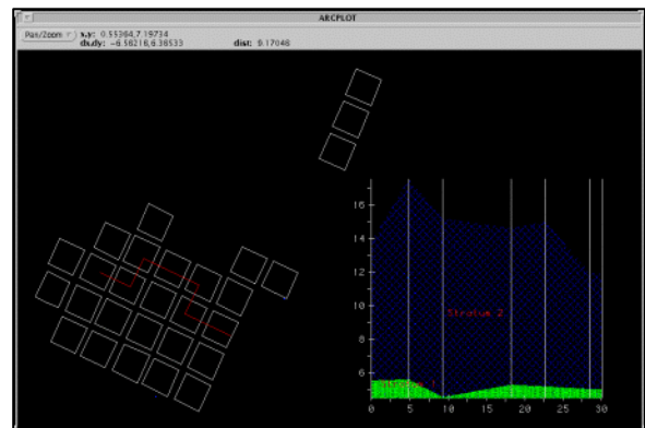
Figure 6. Stratigraphy.
