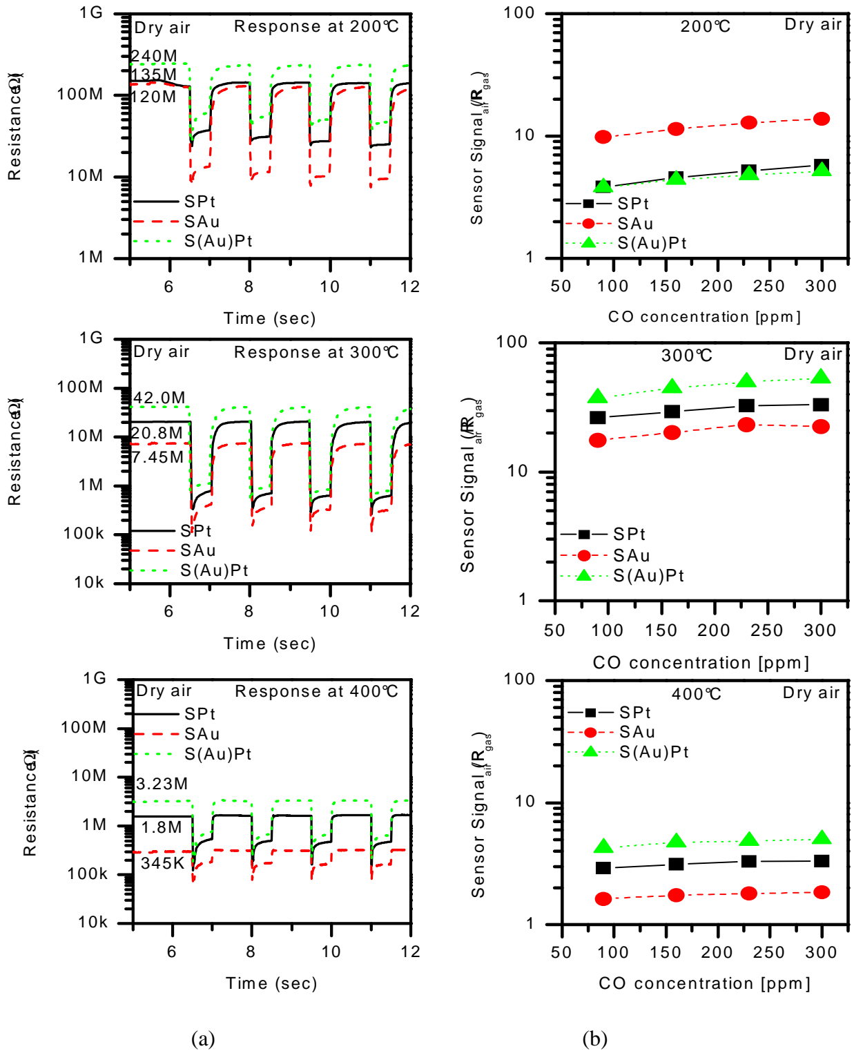
Figure 2-15 : Response (a) and sensor signal of SnO 2 sensor provided with gold electrodes(SAu) or platinum electrodes (SPt) and SnO 2 +1%Au sensor based provided with platinum electrodes (S(Au)Pt) to CO (90,160,230, 300 ppm)in dry air at 200°C, 300°C and 400°C
