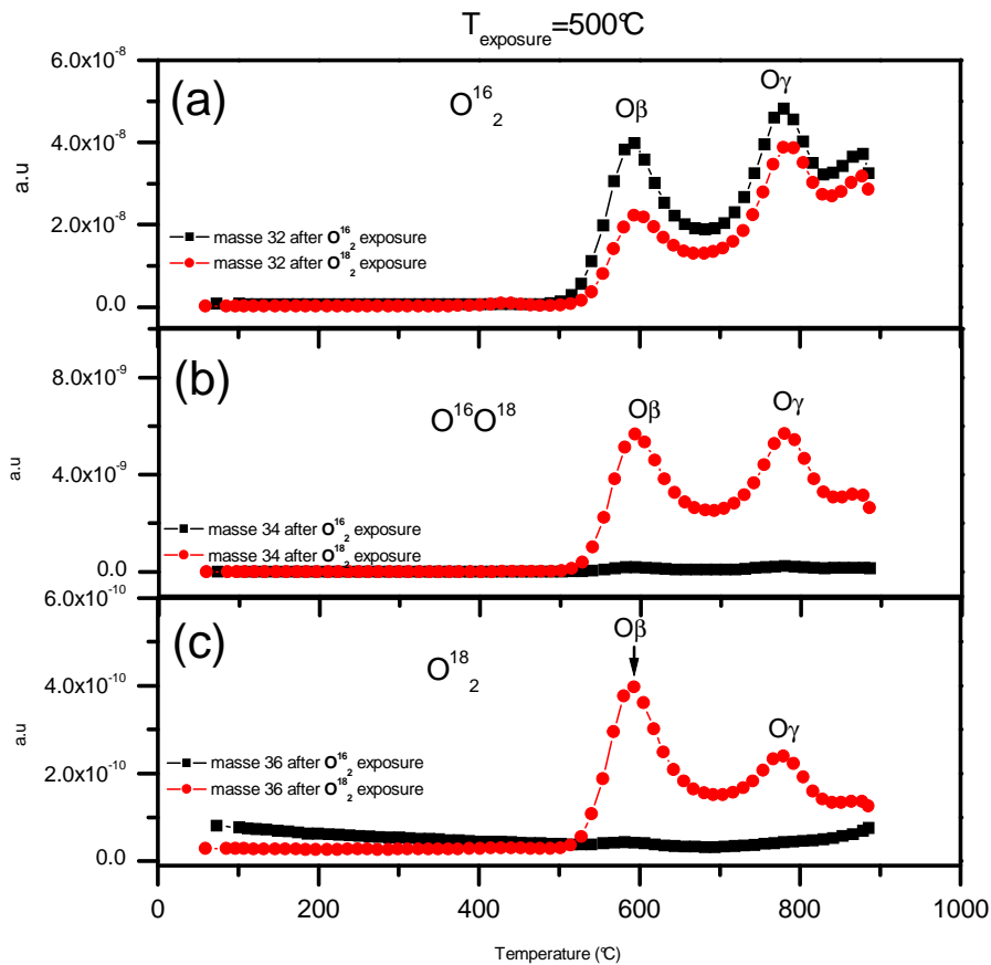
Figure 3-42 : TPD thermogram after exposure to O_2^{18} at 500°C. TPD thermogram with O_2^{16} exposure is used as reference. a) m/e=32 b) m/e=34 c) m/e=36
