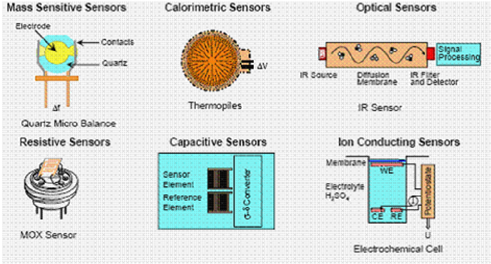
Figure 1-1 : An illustrated selection of gas sensor types
