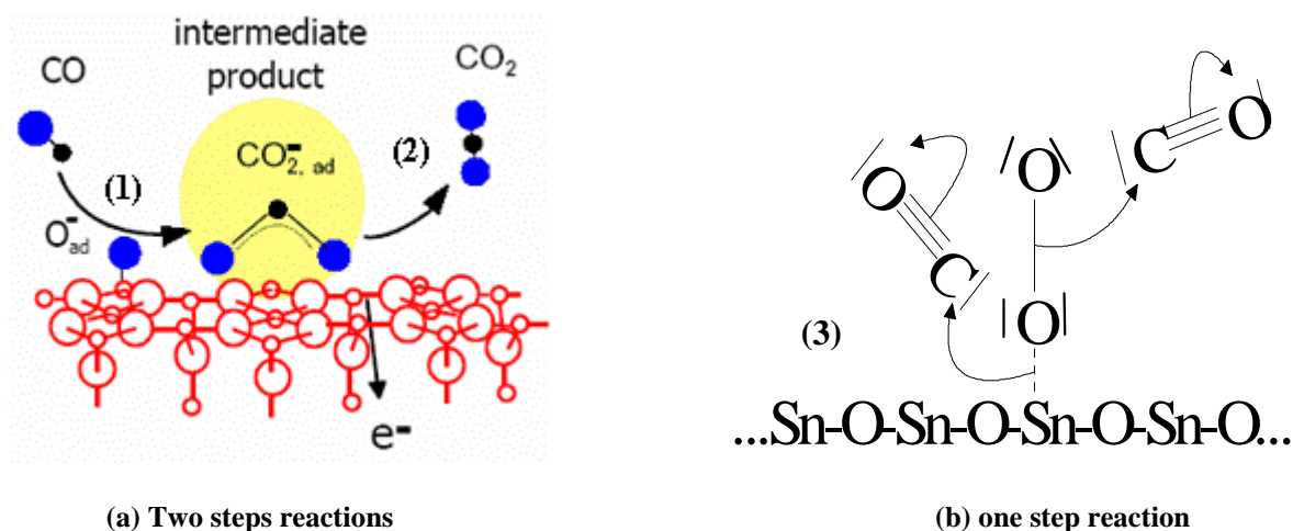
Figure 3-8 : Cartoon of the formation of CO 2 -
