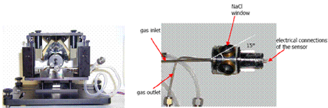
Figure 3-4°: The experimental setup for simultaneous DRIFT, resistance and combustions measurements
