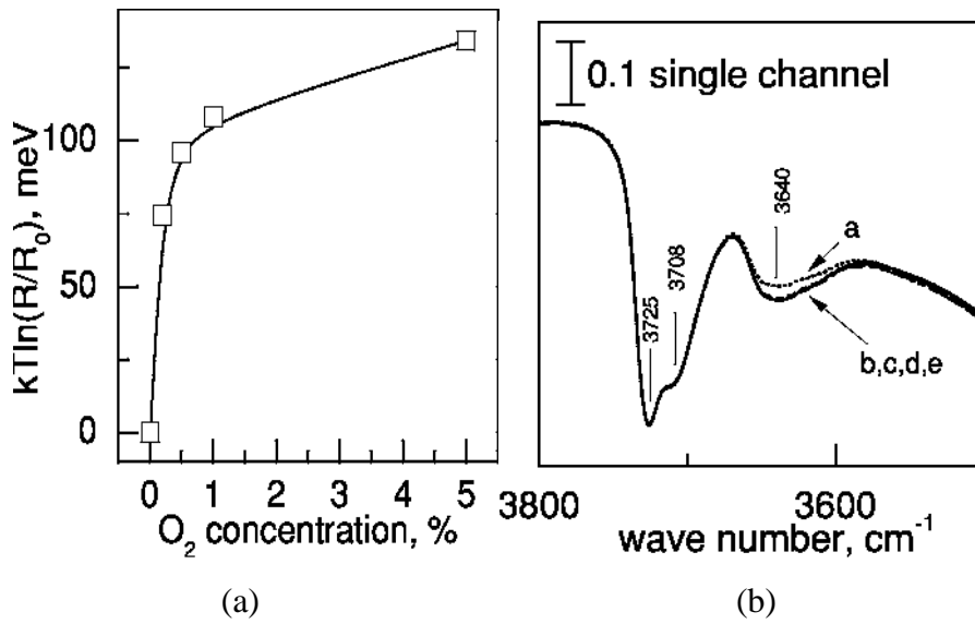
Figure 3-41 :Changes of the band bending (a) and the respective single channel DRIFT spectra (b) of the tin dioxide sensor (U500Y) exposed to oxygen: a - 70 ppm, b - 2 000 ppm, c - 5 000 ppm, d - 10000 ppm, e - 50000 ppm at 400°C and at constant humidity level (3 ppm)[150].
