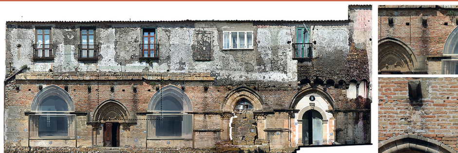
Orthophoto from high resolution camera - facade and details
